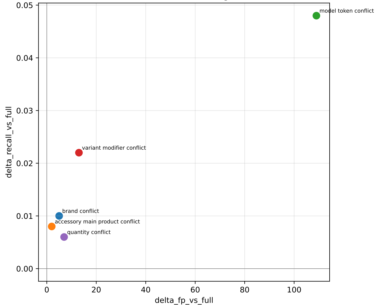
Ablation tradeoff when removing a rule (valid)
