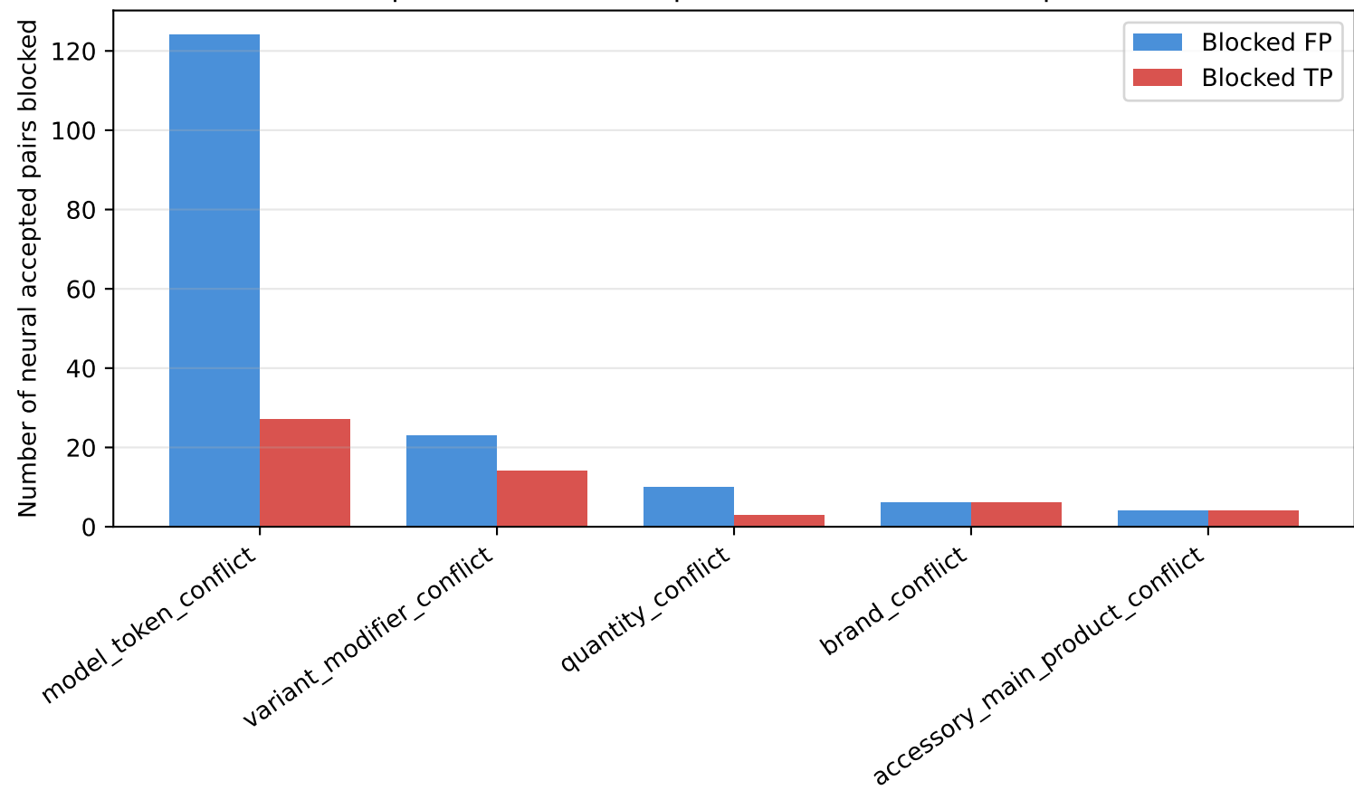
Constraint impact: blocked false positives vs blocked true positives (valid)
