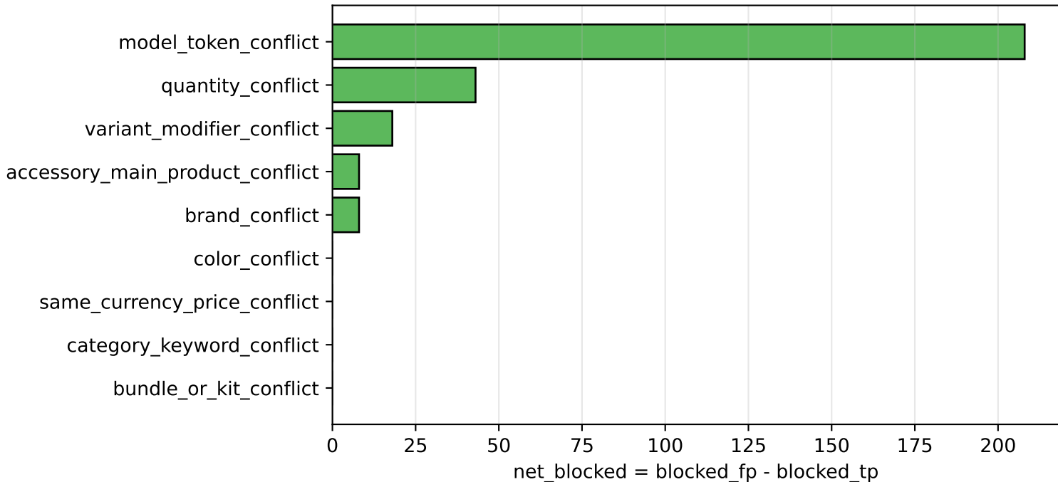
Net symbolic veto effect by constraint (test)
