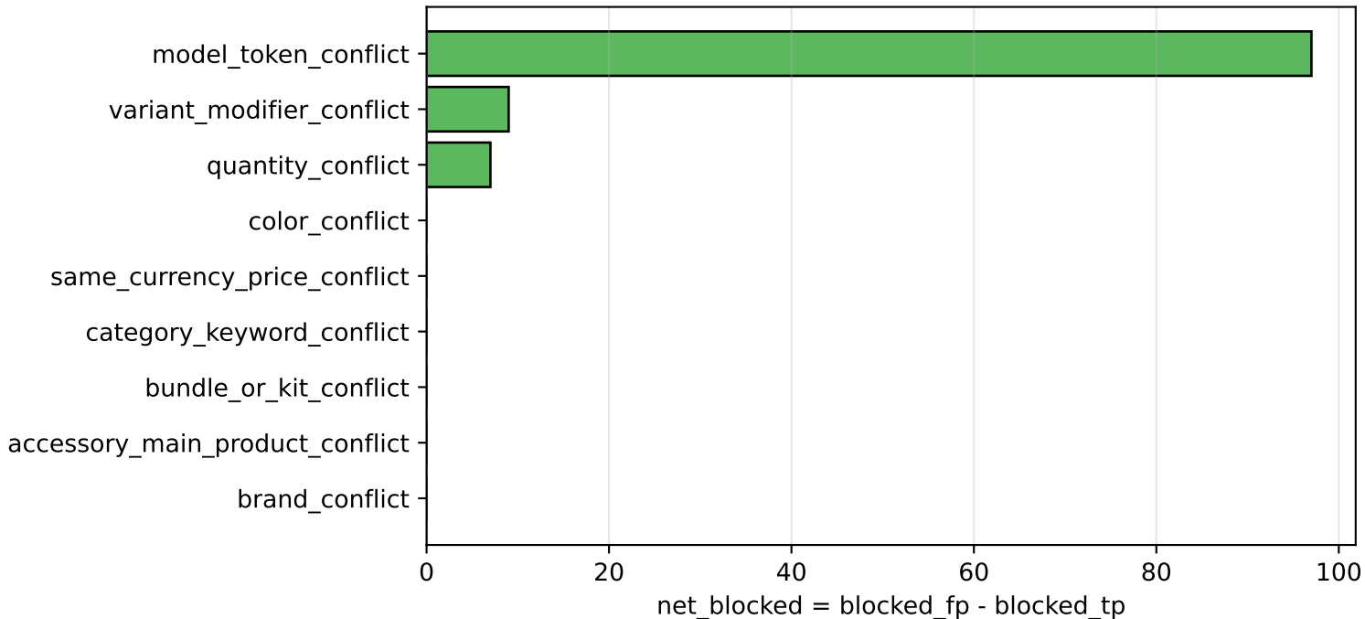
Net symbolic veto effect by constraint (valid)
