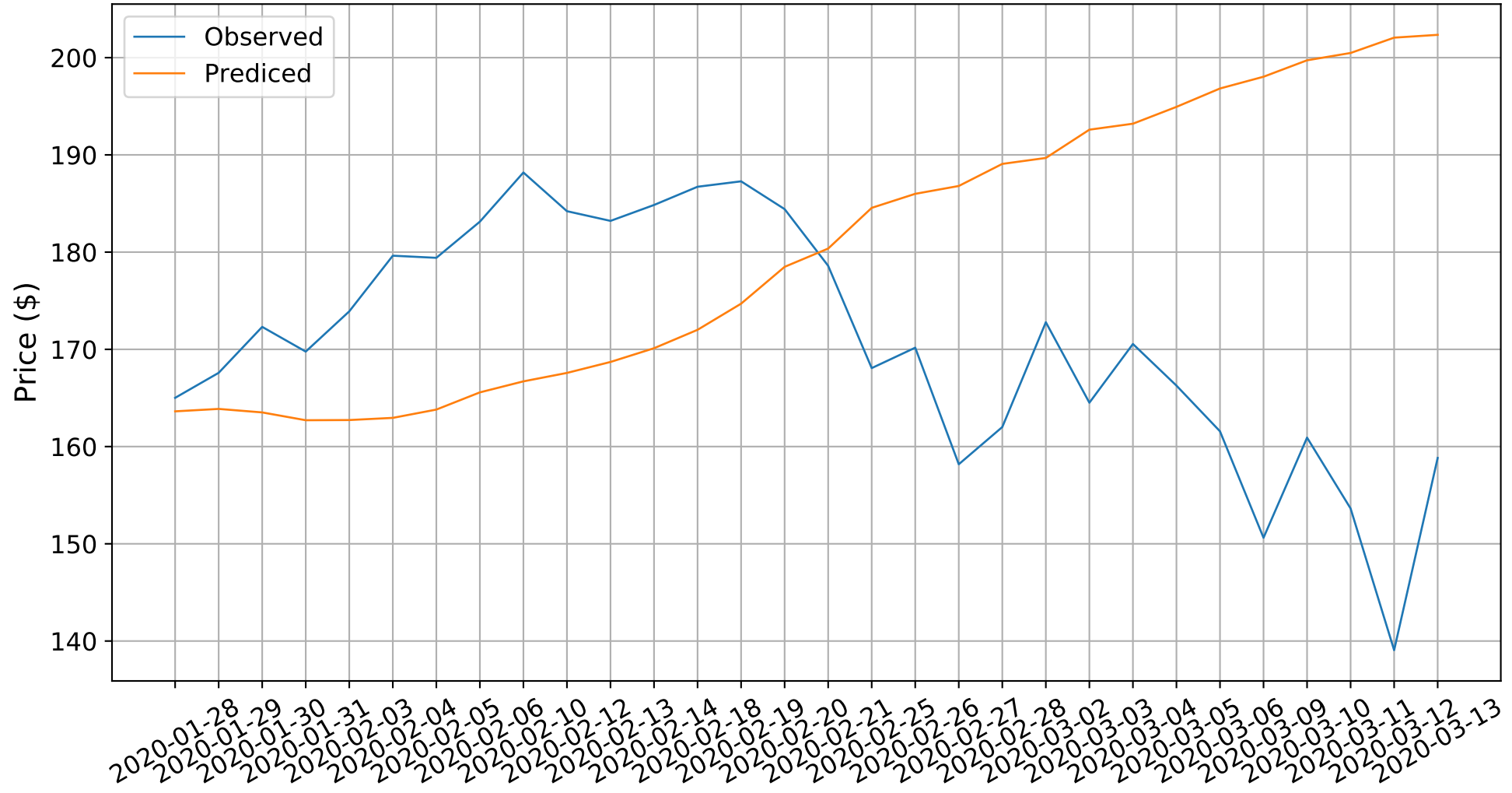
Stock price prediction using linear regression | RMSE = 25.9577
