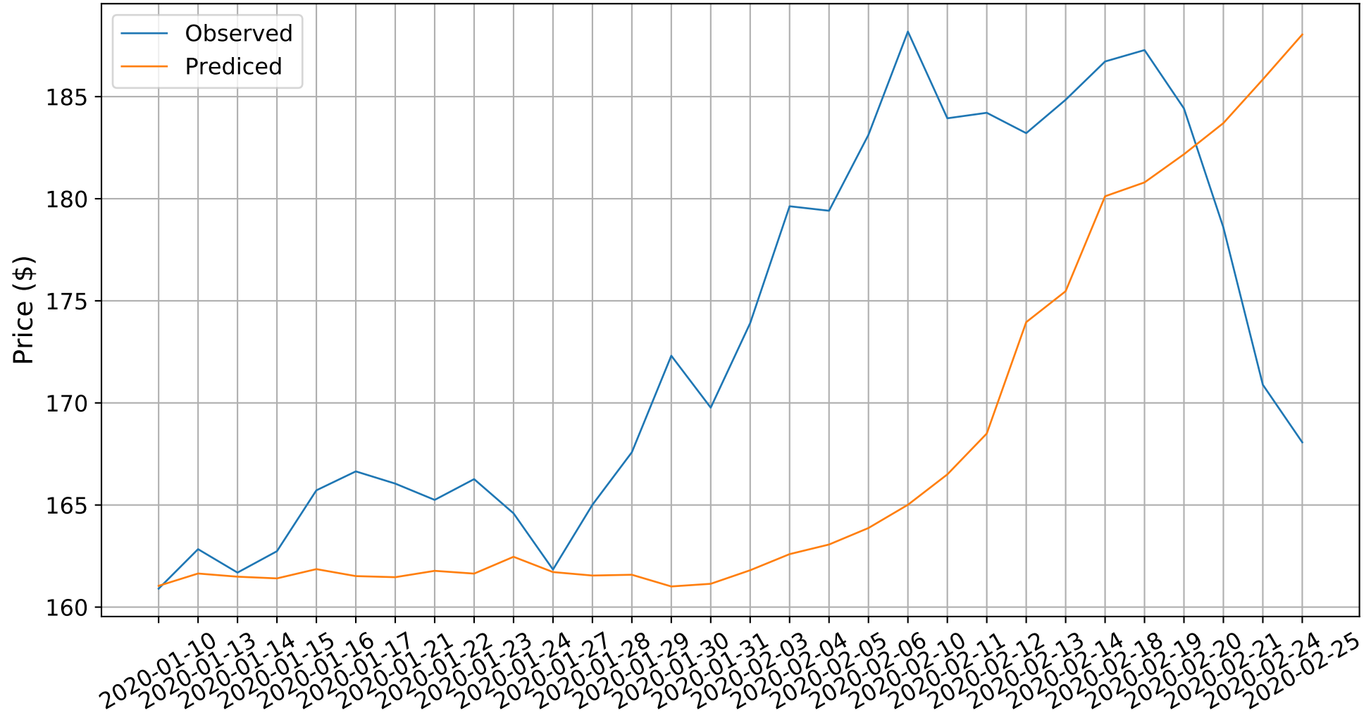
Stock price prediction using linear regression | RMSE = 10.6916
