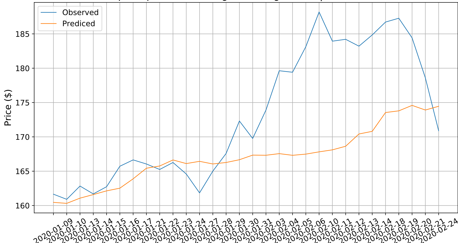
Stock price prediction using linear regression | RMSE = 8.9891
