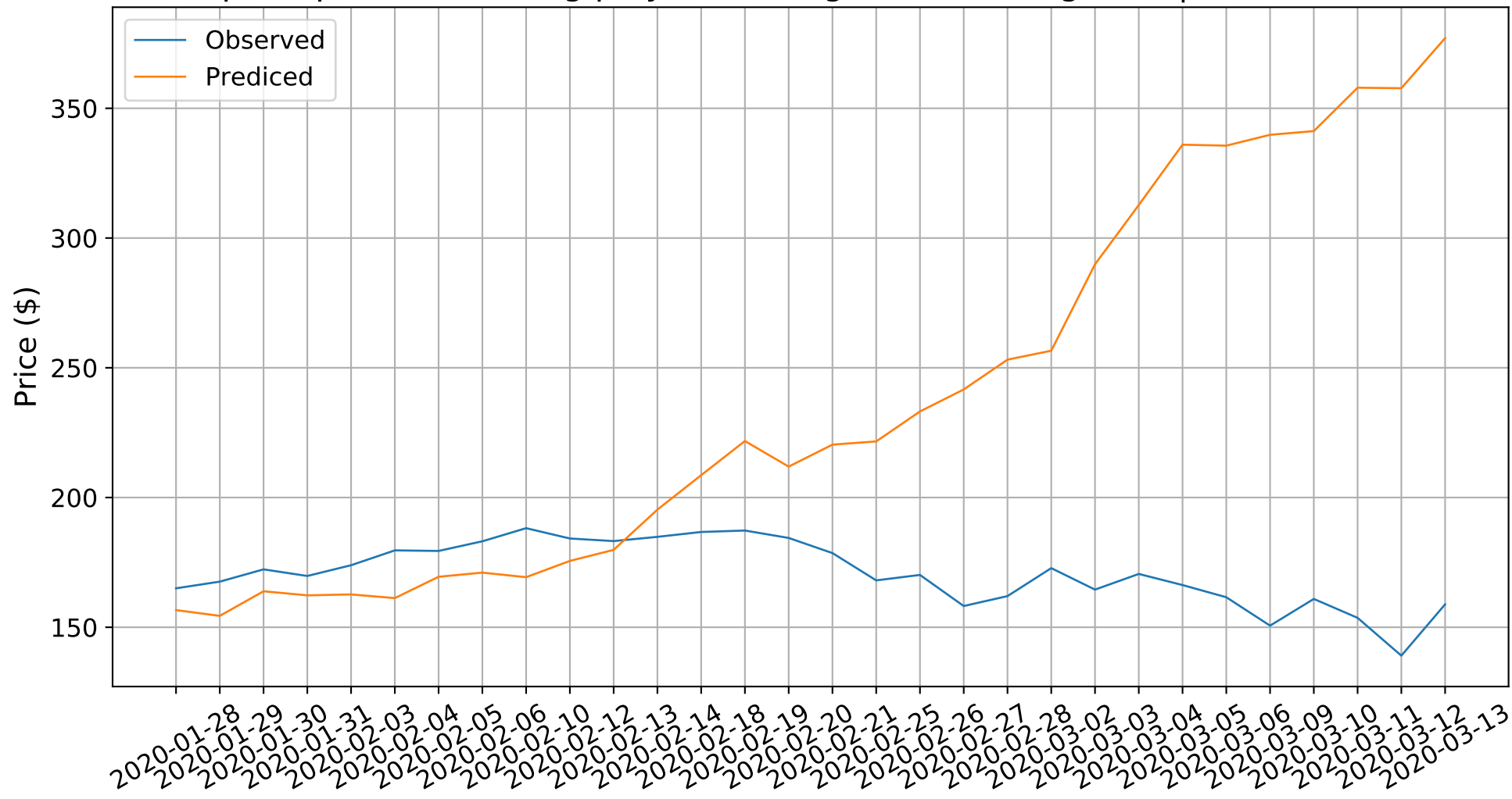
Stock price prediction using polynomial regression of degree 2 | RMSE = 105.7386
