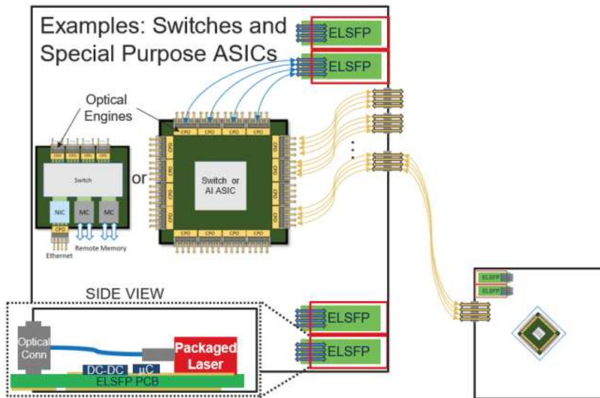
Figure 2 ELSFP in a co-packaged optics application
