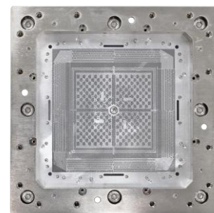
PROBE CARD/SOCKET
