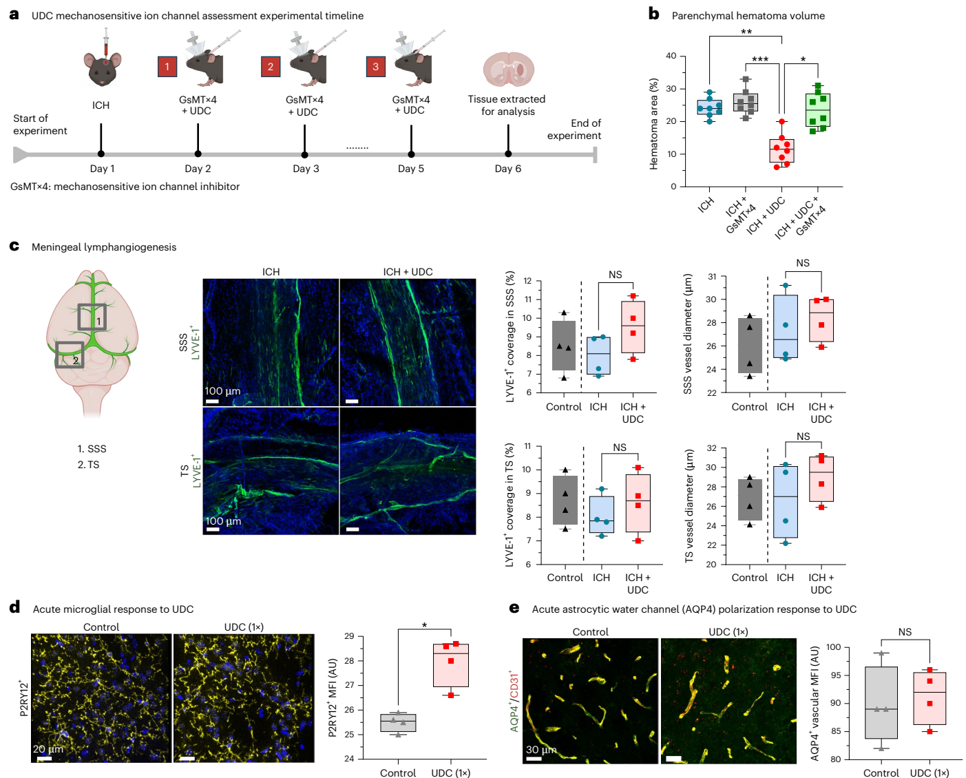
Fig. 6 | UDC is reversed by a mechanosensitive ion channel blocker. a , Timeline of ICH experiment with UDC and a mechanosensitive ion channel blocker (GsMTx4). b , Administration of GsMTx4 reduced the blood product clearance of UDC, as assessed by hematoma volumes across treatment groups. c , Immunohistological analysis of meningeal lymphangiogenesis (LYVE-1 + ) revealed no significant difference between control, ICH + sham and ICH + UDC during this timeline of injury and treatment; SSS, superior sagittal sinus; TS, transverse sinus; NS, not significant. d , In healthy, uninjured mice, immunohistological analysis of purinergic receptors (P2RY12 + , yellow) that
