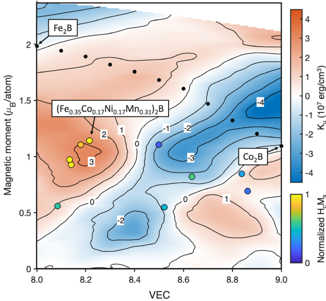
FIGURE 5 | Map of the calculated magnetic anisotropy K_u in (\text{Fe}_{1-x}\text{Co}_x)_2\text{B} as a function of the VEC and average moment of TM species, replotted from Ref. [52]. The black circles are the values calculated for (\text{Fe}_{1-x}\text{Co}_x)_2\text{B} [52]. The colored circles represent selected (\text{Fe}_x\text{Co}_y\text{Ni}_z\text{Mn}_{1-x-y-z})_2\text{B} samples measured at 5 K in the present work. The average TM moment is estimated from the M_s extracted via SQUID and VEC from the TM composition extracted via EDX. The circles are colored according to the product of H_c and M_s measured at 5 K.
