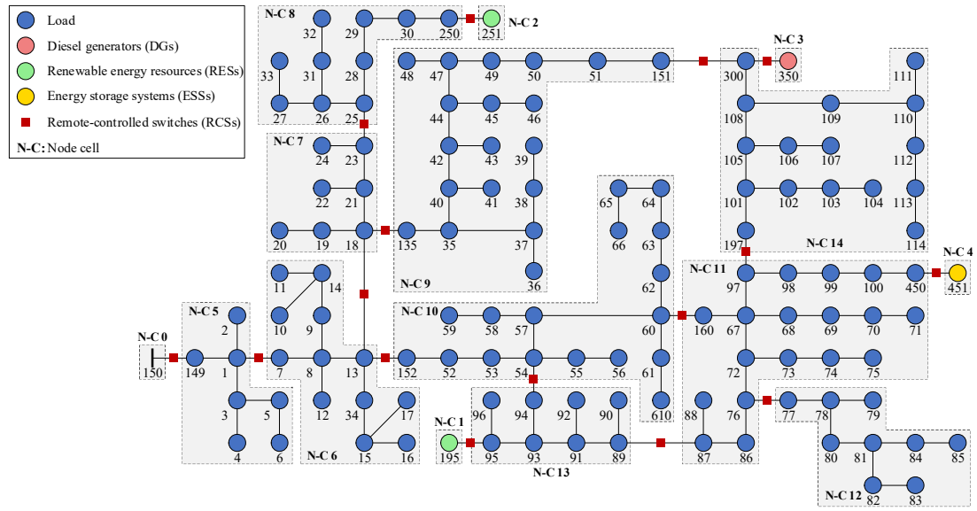
Fig. 1. The modified IEEE 123-node system
