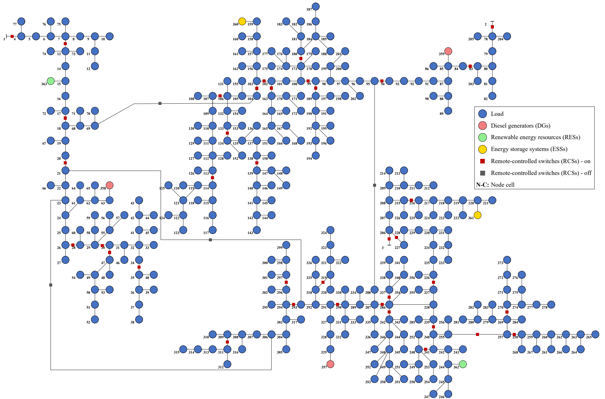
Fig. 2. The modified 356-node regional system in China
