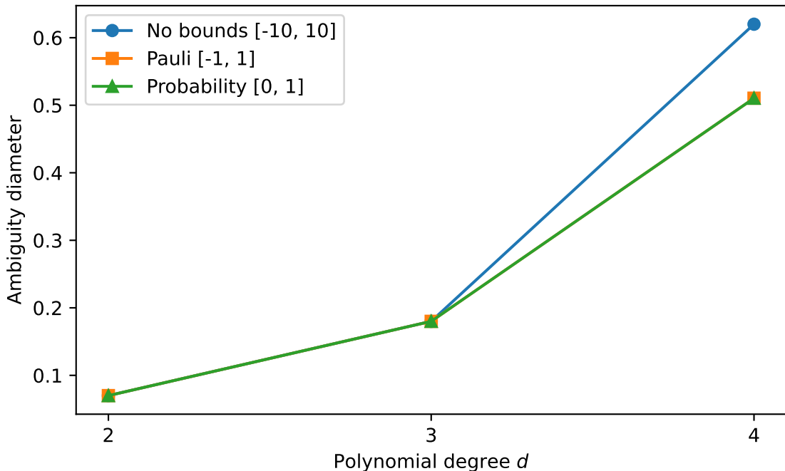
Ambiguity diameter vs model complexity ( n = 5 , \delta = 0.01 )
