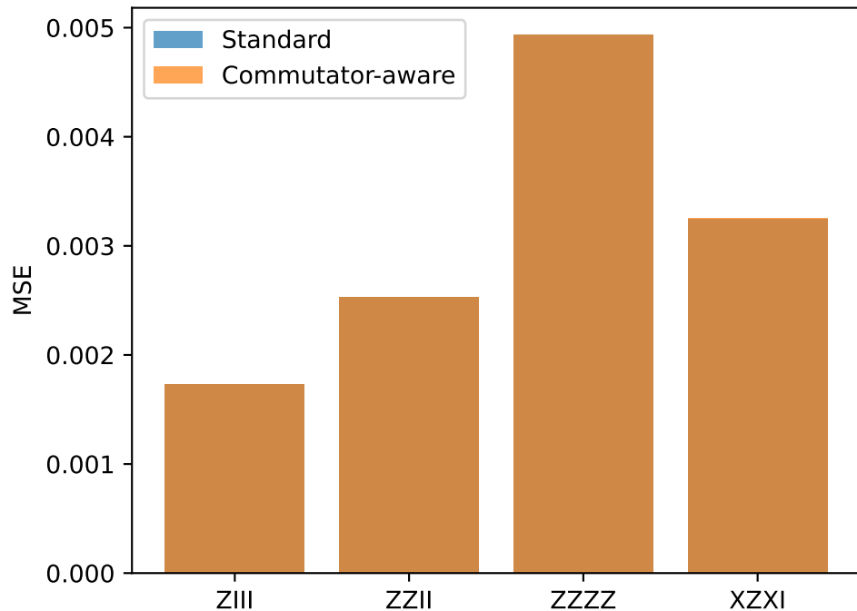
MSE: standard vs commutator-aware
