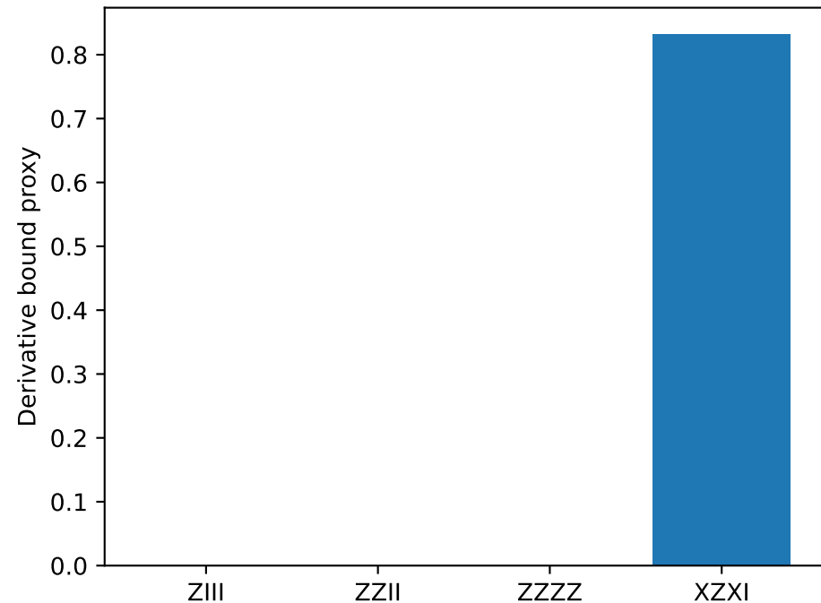
Commutator envelope by observable
