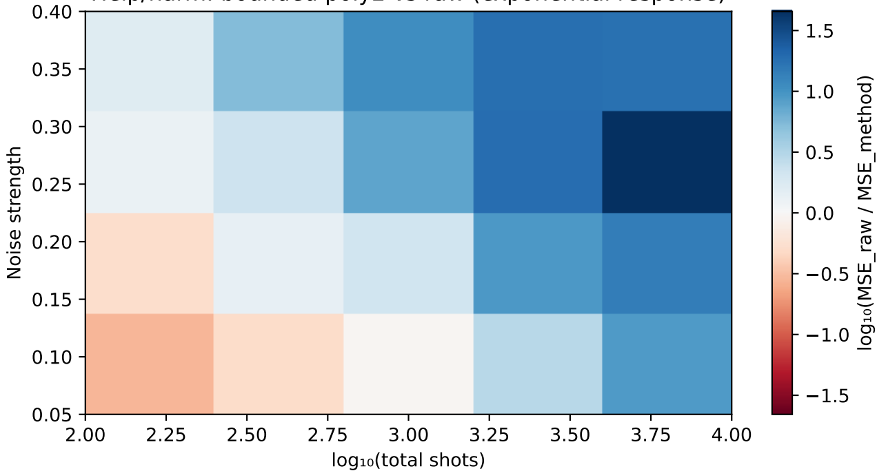
Help/harm: bounded poly2 vs raw (exponential response)
