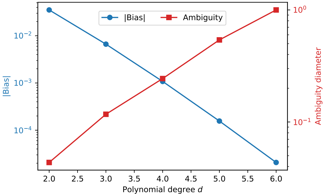
Bias-ambiguity tradeoff ( n = 7 , \delta = 0.01 , bounds [0, 1] )
