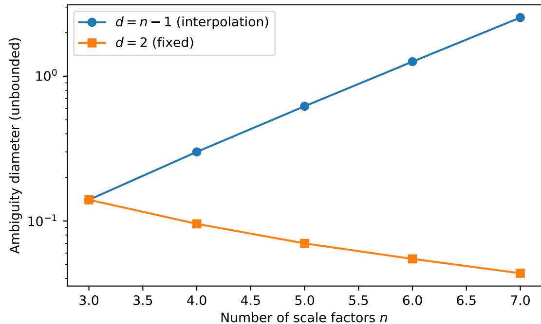
n-sensitivity: interpolation vs fixed degree ( \delta = 0.01 )
