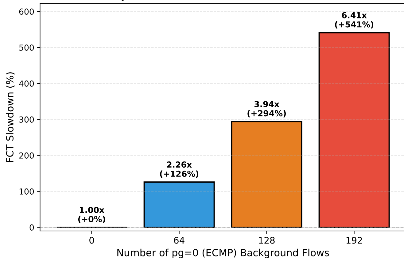
8KB MoE Flow: FCT Slowdown vs FECMP Background Flows (Hybrid Mode, IRN-PFC, fat-k8-100G-OS10)
