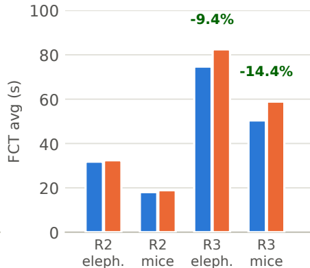
(c) Flow completion time (avg)
