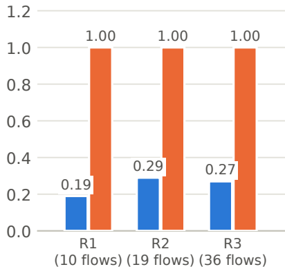
(a) Per-flow spine skew (mean)
