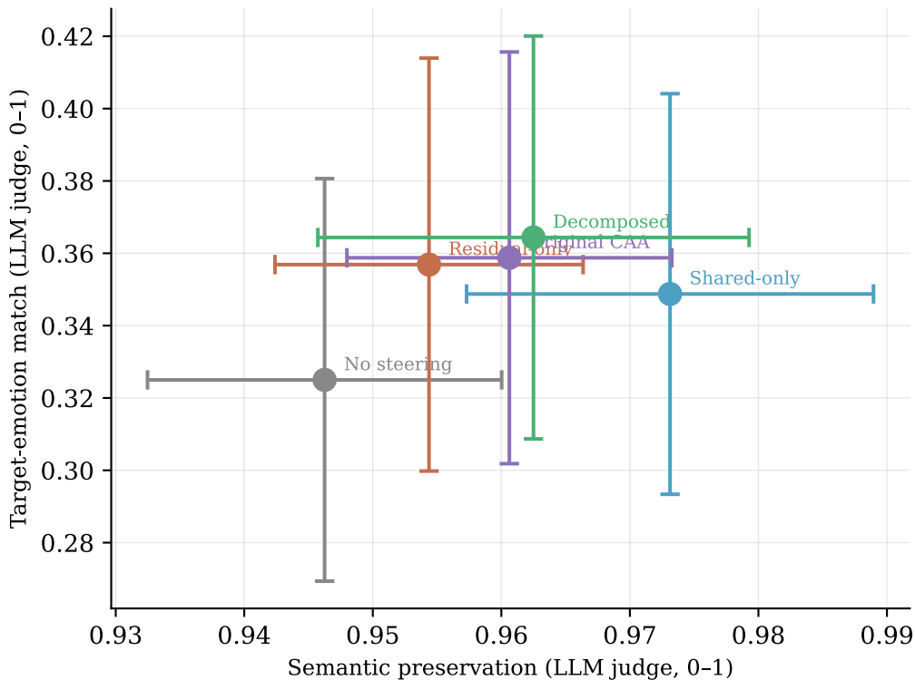
Semantic preservation vs. target-emotion match (error bars = 95% CI, n=160 per condition)
