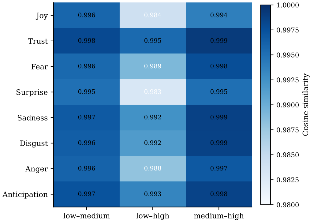
Intensity-pair cosine similarity per emotion (Layer 13)
