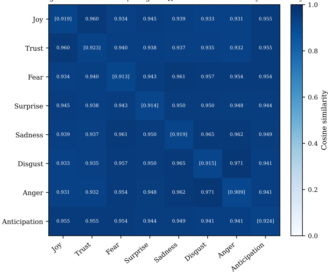
Source-paired cosine similarity of CAA directions (Layer 13)
