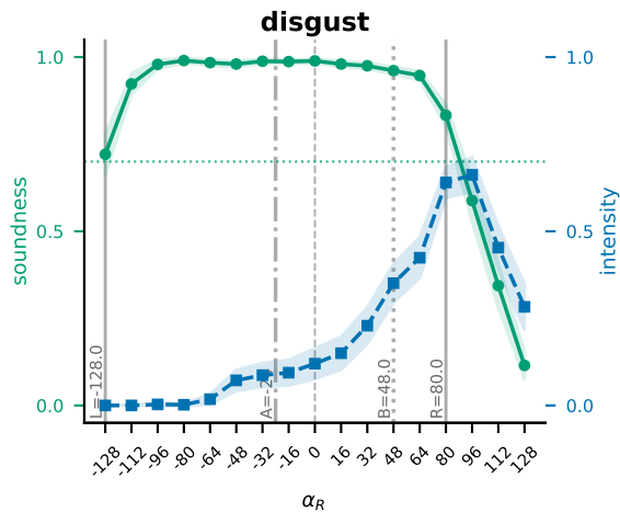
Coherence thresholds and midpoints per emotion ( \alpha_G = 0 )
