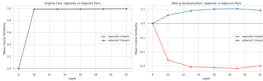
Figure 3.6: Mean cosine similarity of Plutchik opposite and adjacent emotion pairs across layers, before and after g -residualisation.
