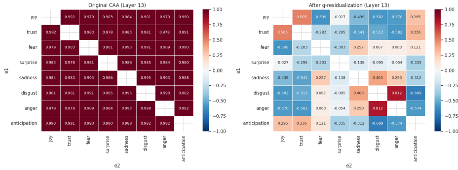
Figure 3.4: Original vs g-residualised cosine heatmap
