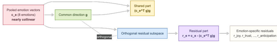
Figure 3.5: Decomposition of CAA vectors into a shared emotionalisation component g and emotion-specific residuals r_e . The original pooled CAA vector c_e is the sum of these two components. This decomposition reveals that while the dominant structure is a common shift towards emotionality, there is also a structured residual geometry that encodes specific emotion identities.
