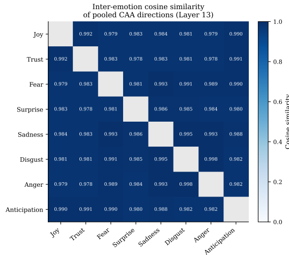
Figure 3.5: Inter-emotion cosine similarity of pooled CAA vectors at layer 13. The colour scale spans [0, 1] ; all off-diagonal entries lie above 0.97, indicating that every emotion pair shares a dominant common component.
