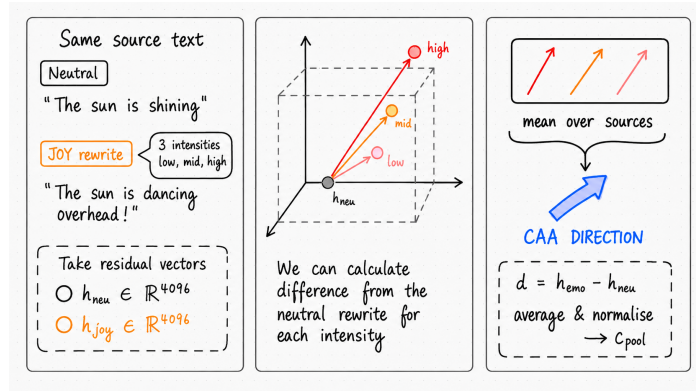
Figure 3.4: Schematic overview of CAA vector construction.
