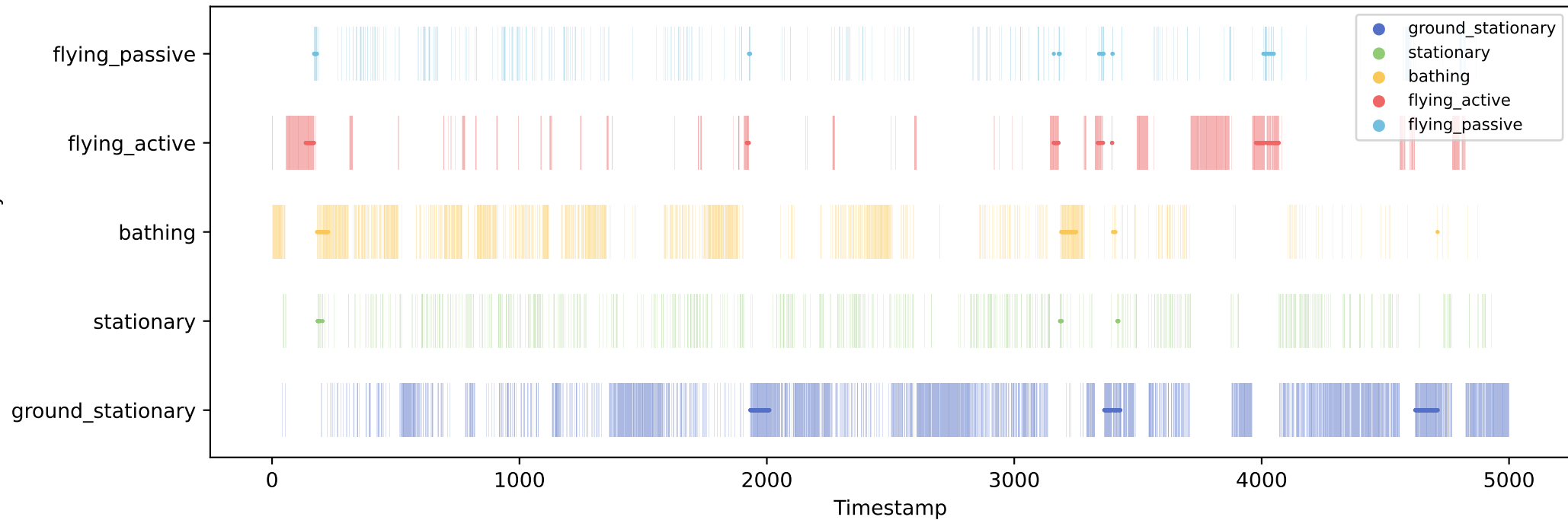
Groundtruth (lines) vs Propagated labels (rectangles)
