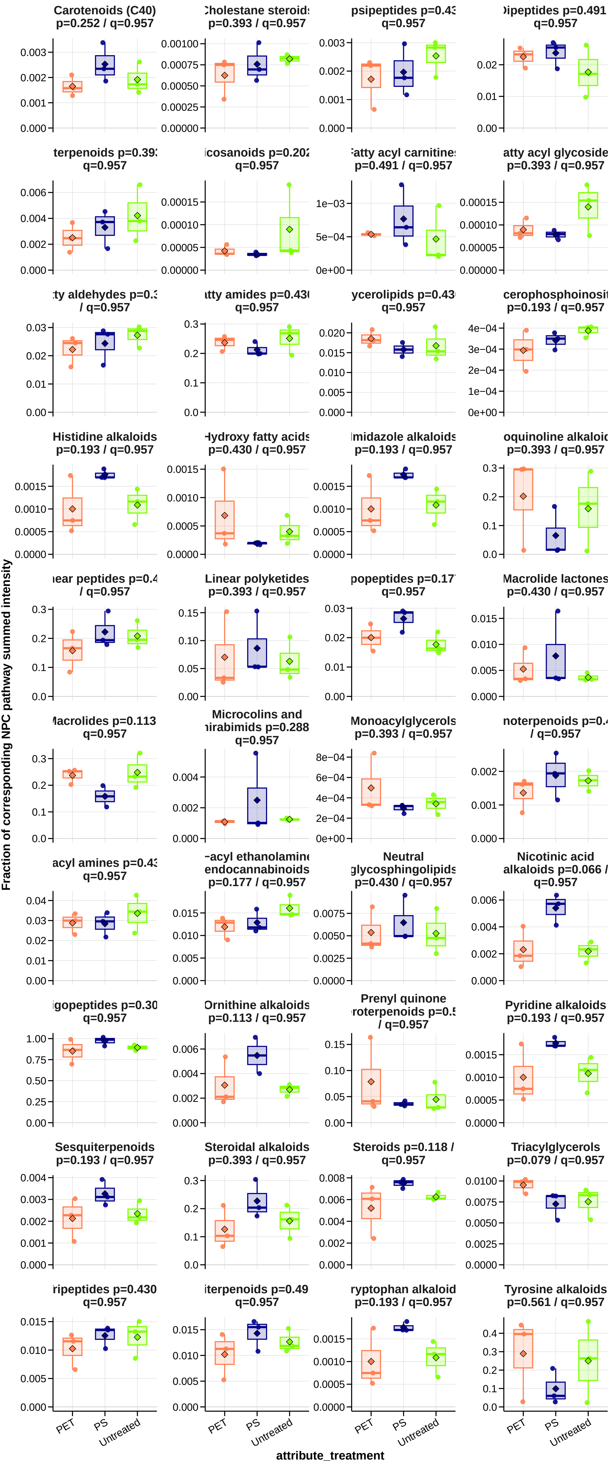
Top 40 NPC class/superclass pathway-normalized intensities for mapp_batch_00268 (raw data)
