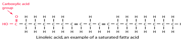
Figure 5.4: http://hyperphysics.phy-astr.gsu.edu/hbase/Organic/imgorg/linoleic.png
