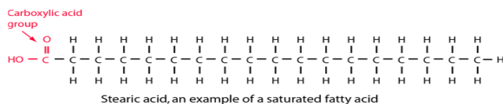
Figure 5.3: http://hyperphysics.phy-astr.gsu.edu/hbase/Organic/imgorg/stearic.png
