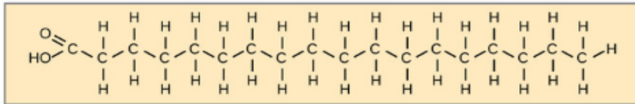
Stearic acid
