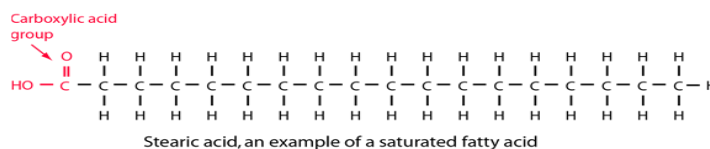
Figure 5.3: http://hyperphysics.phy-astr.gsu.edu/hbase/Organic/imgorg/stearic.png
