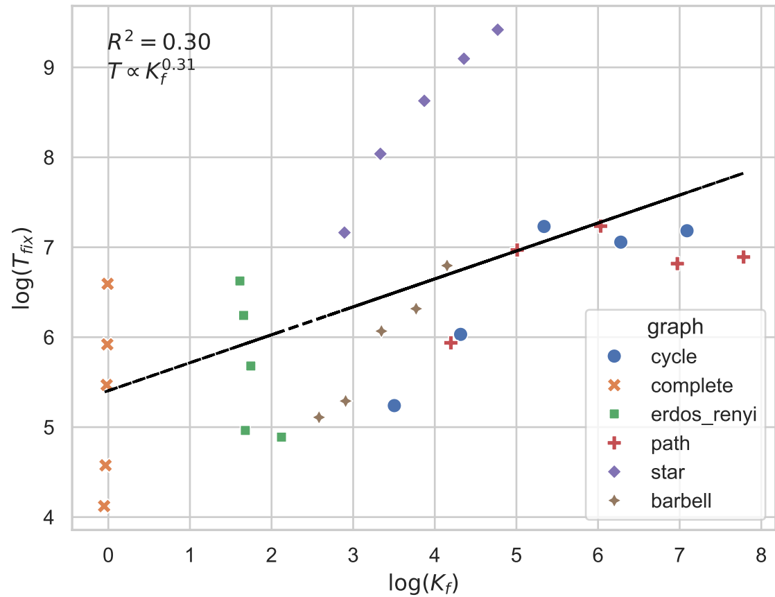
(b) Effective Resistance
