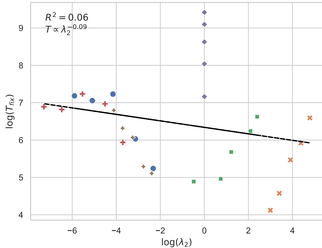
(a) Spectral Gap
