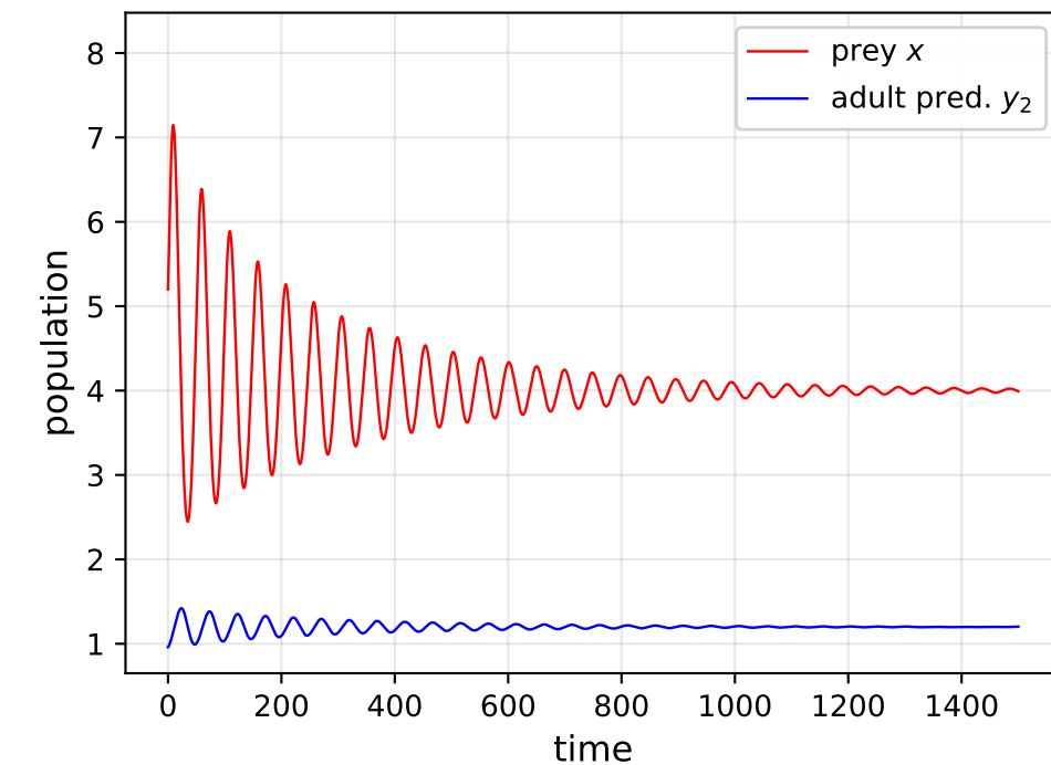
\bar{g} = 0.5 (deterministically stable), v = 0
