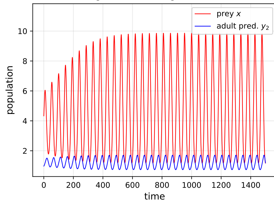
\bar{g} = 0.45 (just above g_1 ), v = 0
