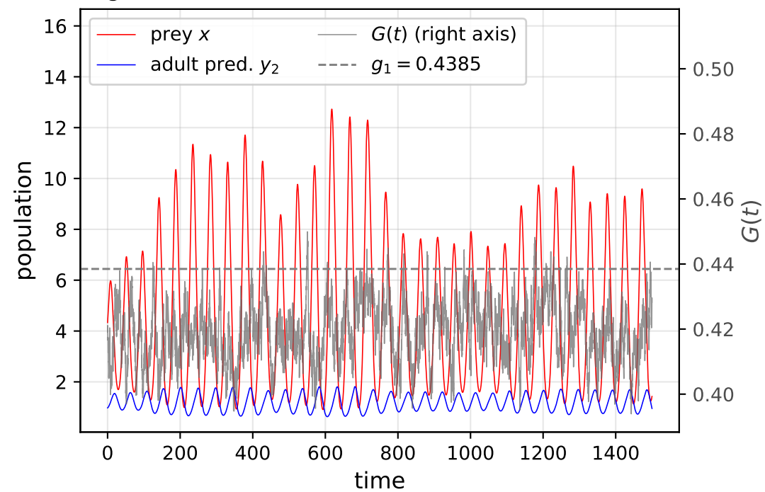
\bar{g} = 0.45, \alpha = 0.133, v = 0.00125, \text{std } G = 0.0106
