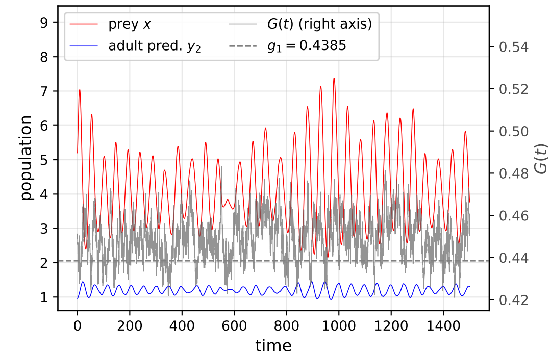
\bar{g} = 0.5, \alpha = 0.133, v = 0.00125, \text{std } G = 0.0124
