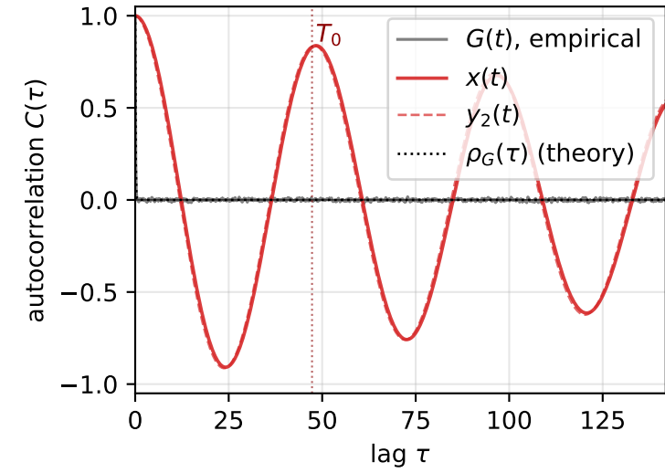
(c) Autocorrelations
