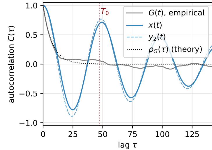
(f) Autocorrelations
