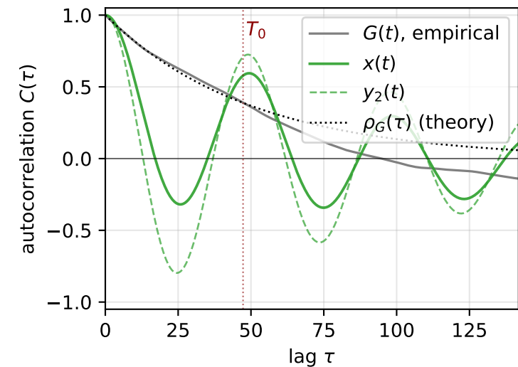
(i) Autocorrelations
