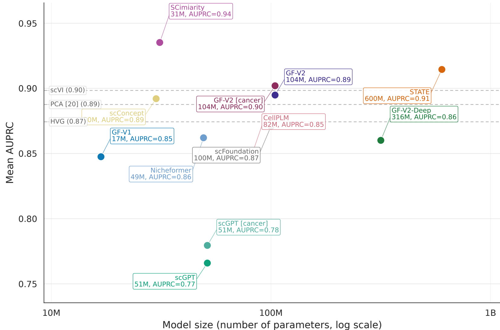
Classification performance vs model size (MIL aggregation)
