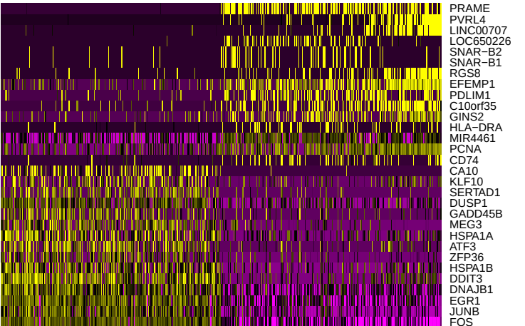
PC_10
