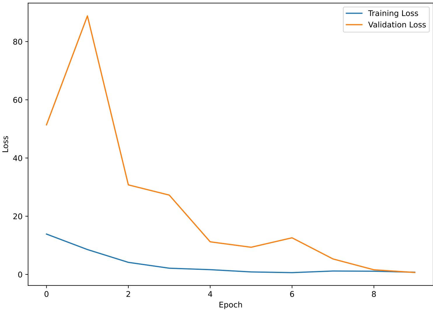
CNN Loss
