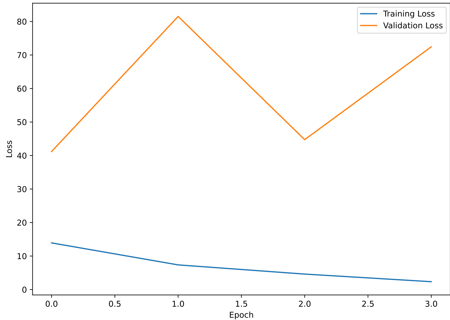
CNN Loss
