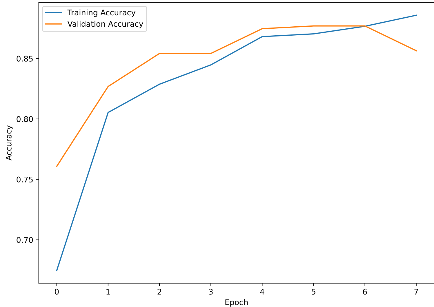
MobileNetV2 Accuracy
