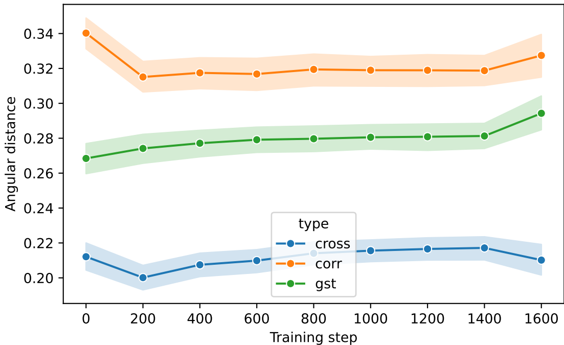
Grad-cross term distances over training (mean over layers, experts)
