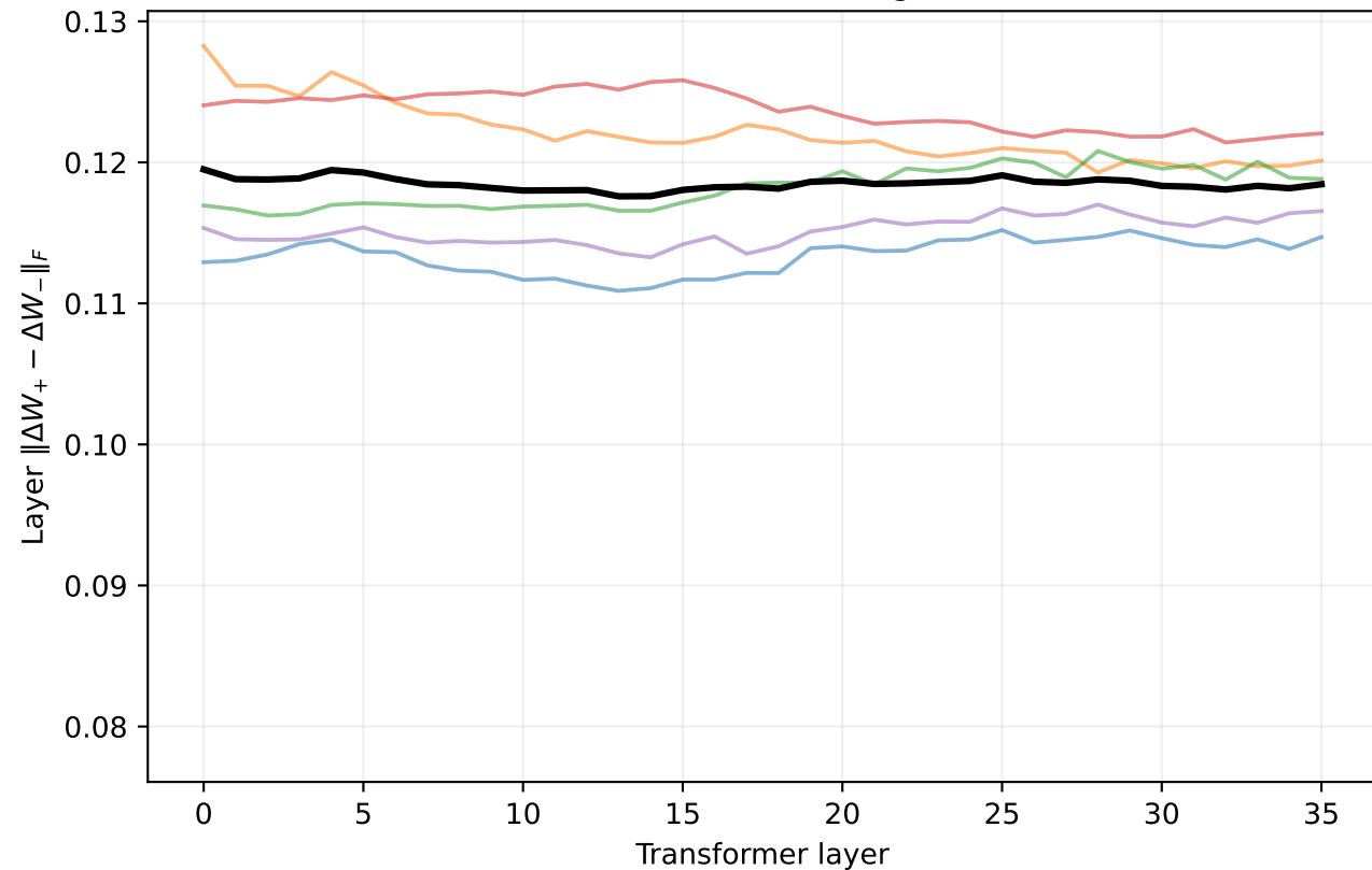
NC: non-cheating
