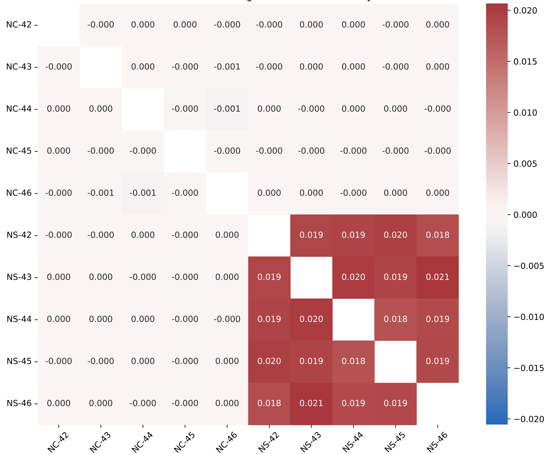
Seeded effective steering-vector cosine similarity
