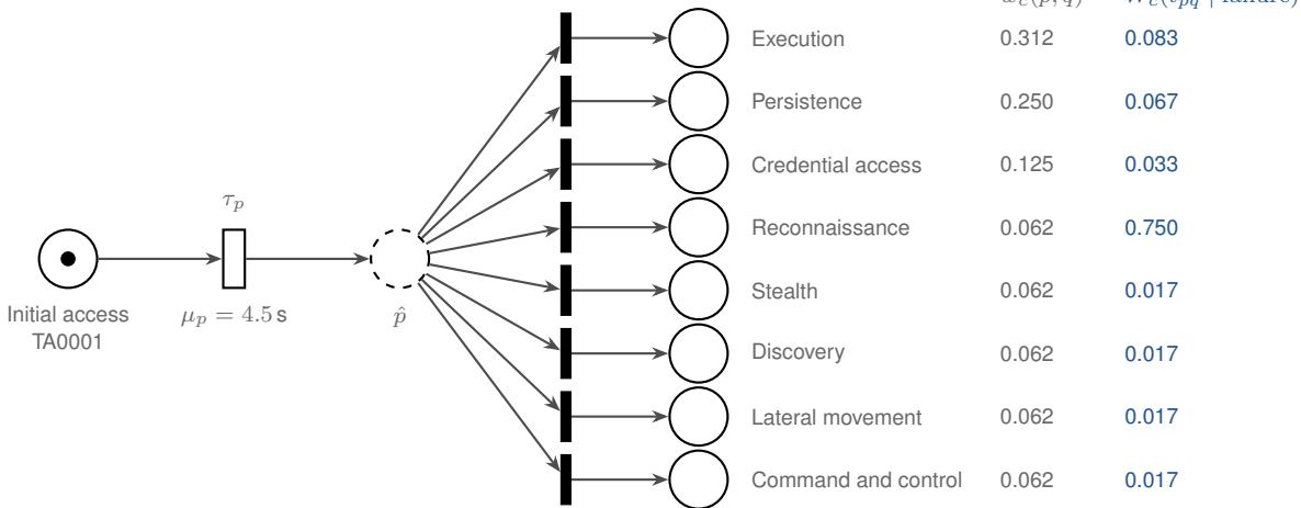
(b) The same gadget on initial access in the exfiltration profile
