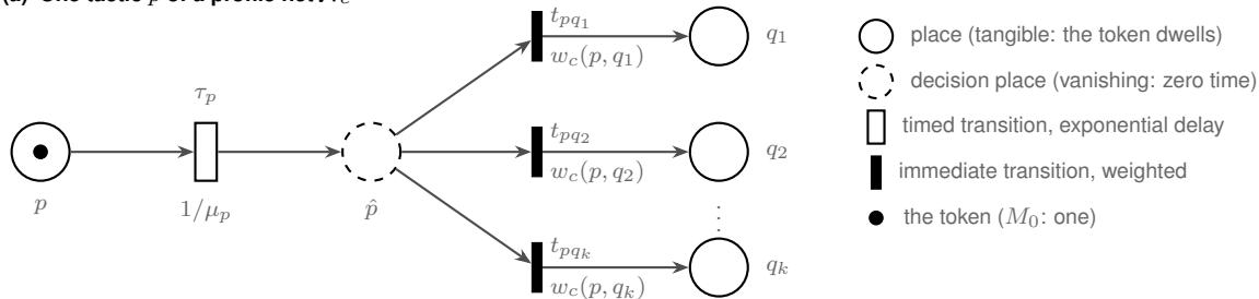
(a) One tactic p of a profile net \mathcal{N}_c
