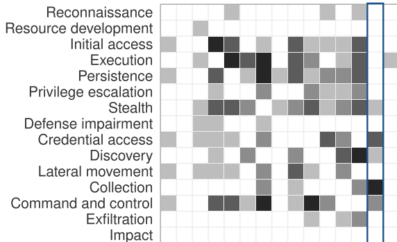
c_1 (19 attack flows)
