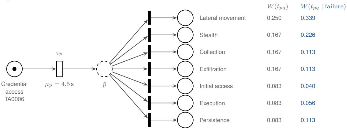
(c) Credential access in c_1
