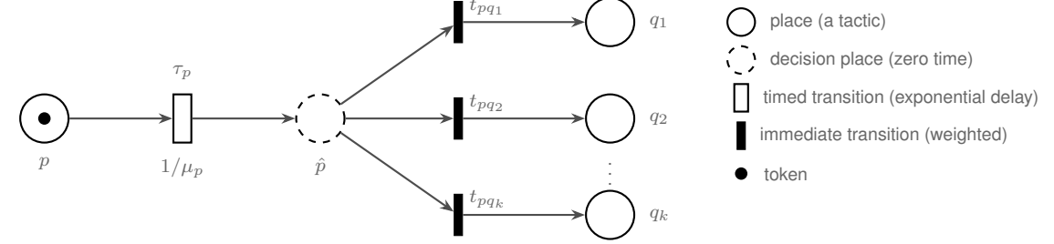
(a) One tactic p of a Petri net \mathcal{N}_c
