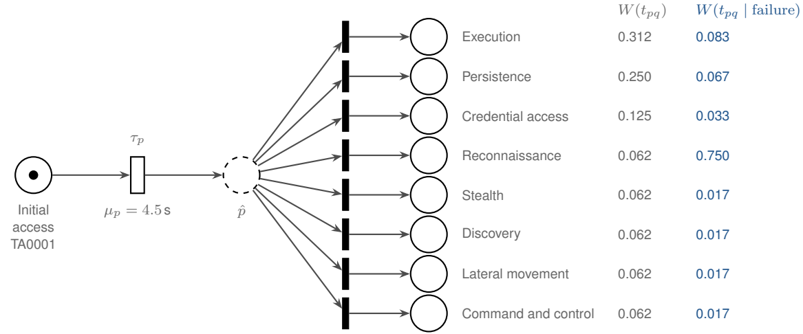
(b) Initial access in c_1
