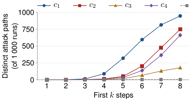
(b) Distinct attack paths
