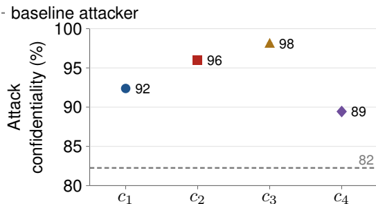
(c) Attack confidentiality
