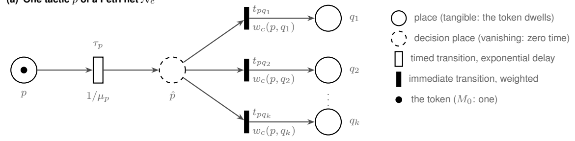
(a) One tactic p of a Petri net \mathcal{N}_c
