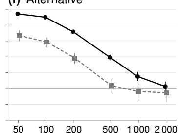
(f) Alternative
