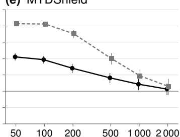
(e) MTDSshield
