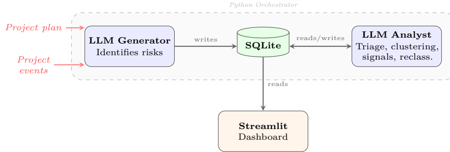
Fig. 1. System architecture. The LLM Generator identifies risks from the project plan and subsequent events; the LLM Analyst reads risks from SQLite, applies triage, clustering, and signal scanning, and writes classifications back. A Python orchestrator (dashed) coordinates the pipeline. The dashboard reads from SQLite for visualization.
