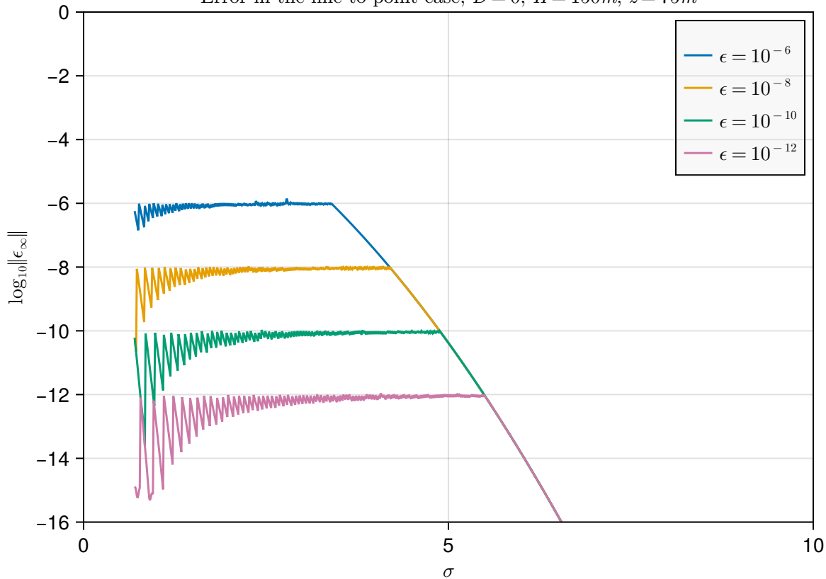
Error in the line to point case; D = 0 , H = 150m , z = 75m
