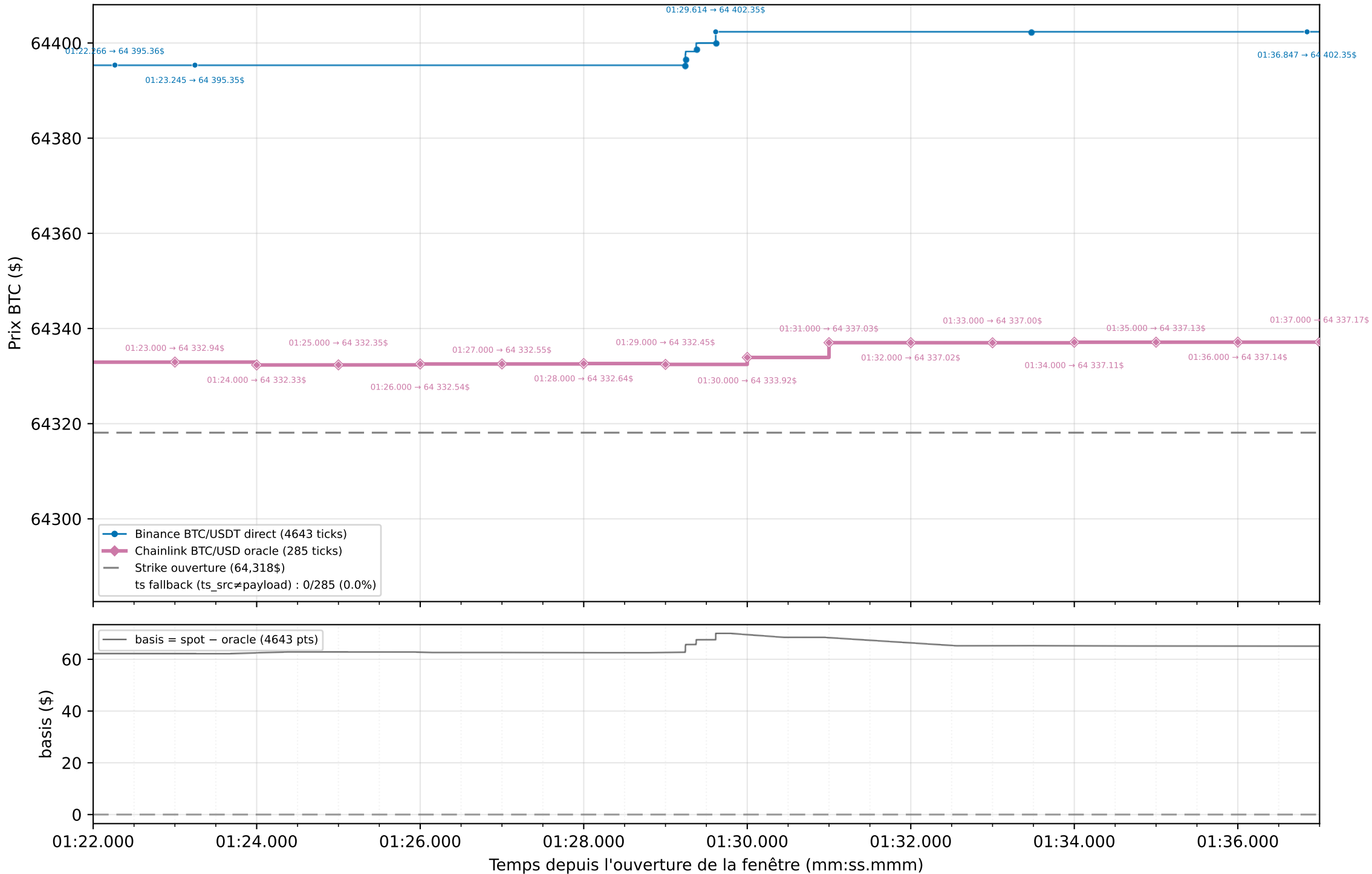
Graphique 2 : Spot Binance (flux direct) vs Oracle Chainlink — strike exact (dernier tick \leq t_0 ) — zoom 15 s [01:22.000 → 01:37.000]
