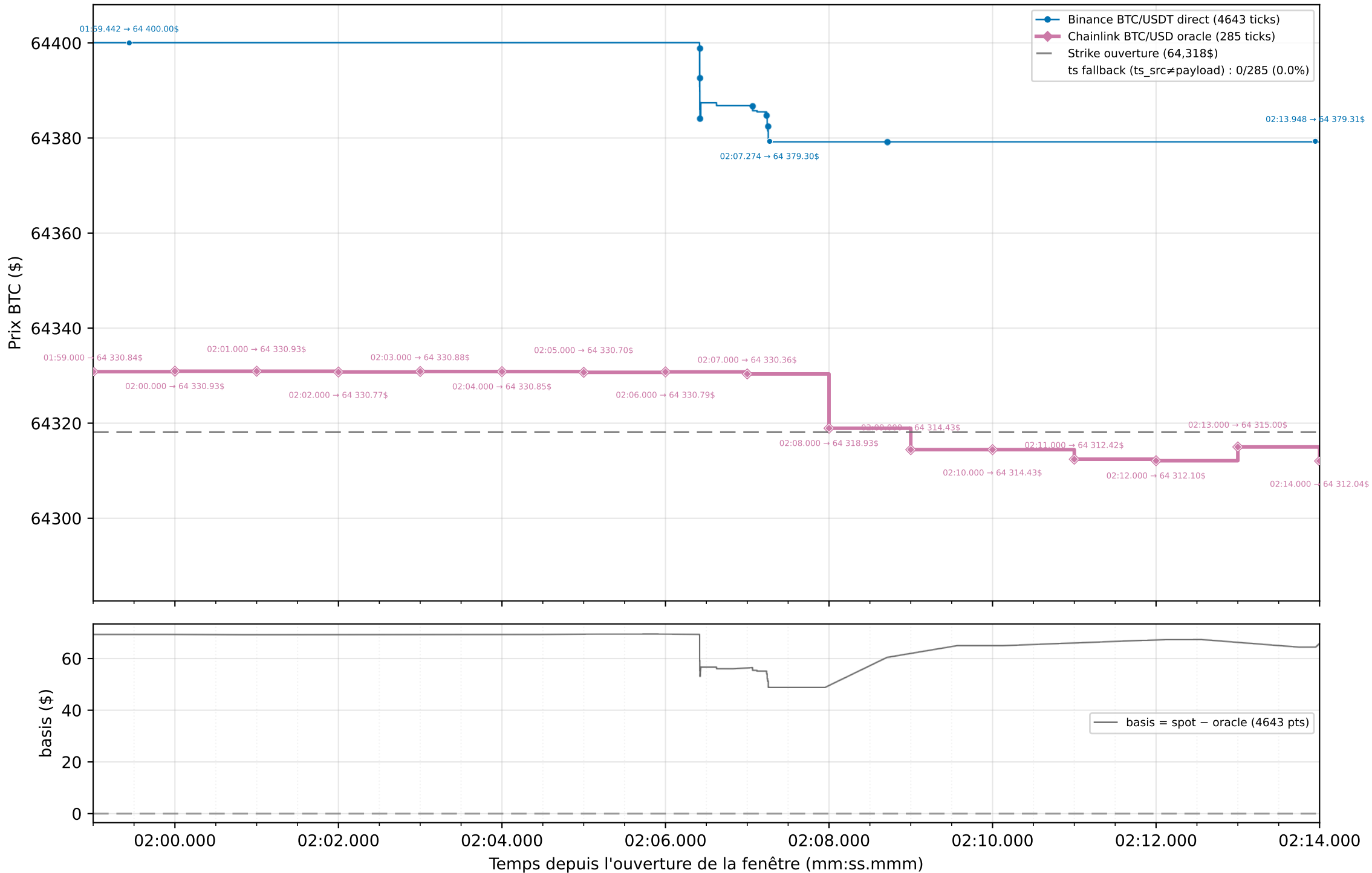
Graphique 2 : Spot Binance (flux direct) vs Oracle Chainlink — strike exact (dernier tick \leq t_0 ) — zoom 15 s [01:59.000 → 02:14.000]
