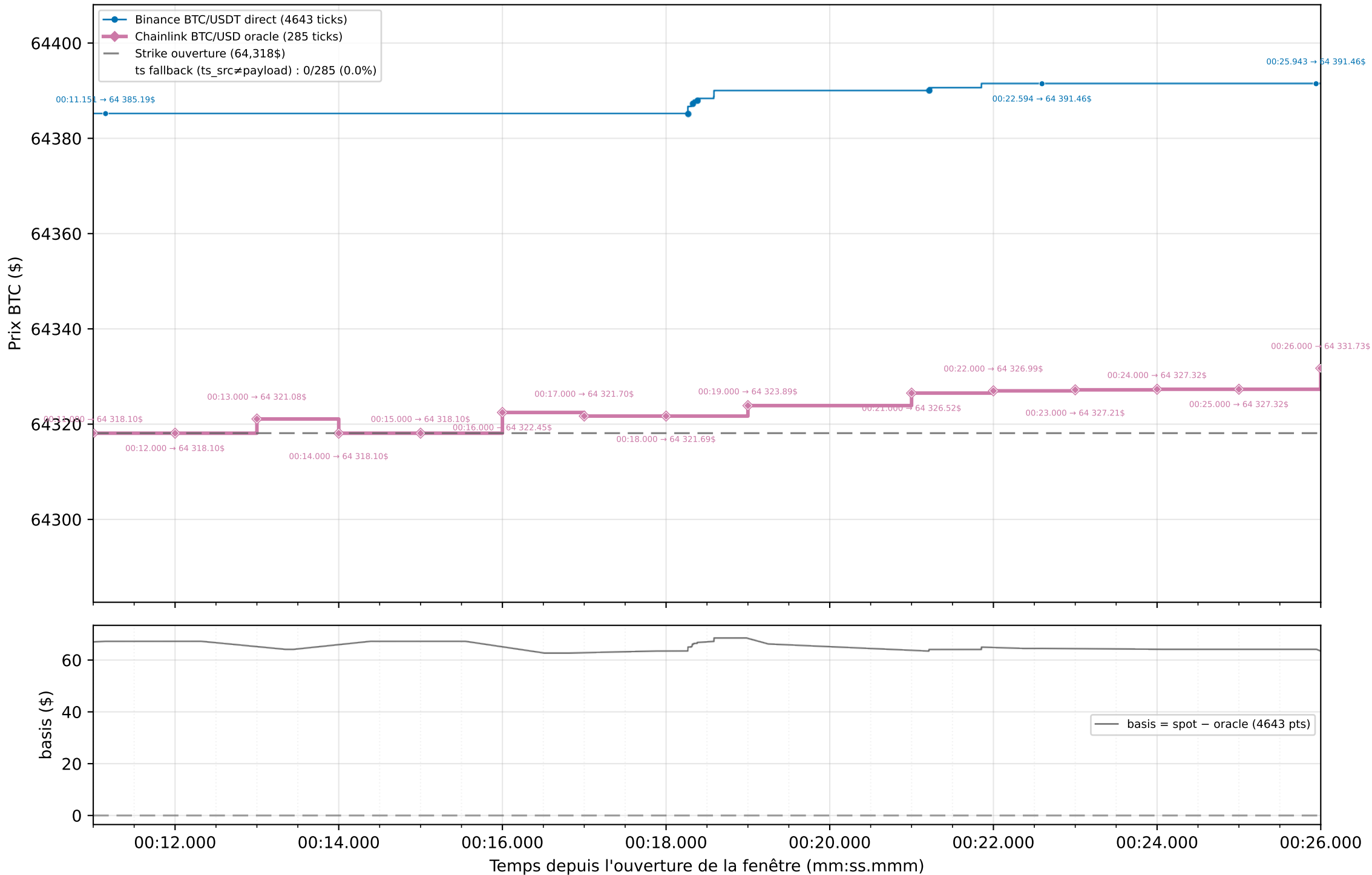
Graphique 2 : Spot Binance (flux direct) vs Oracle Chainlink — strike exact (dernier tick \leq t_0 ) — zoom 15 s [00:11.000 → 00:26.000]
