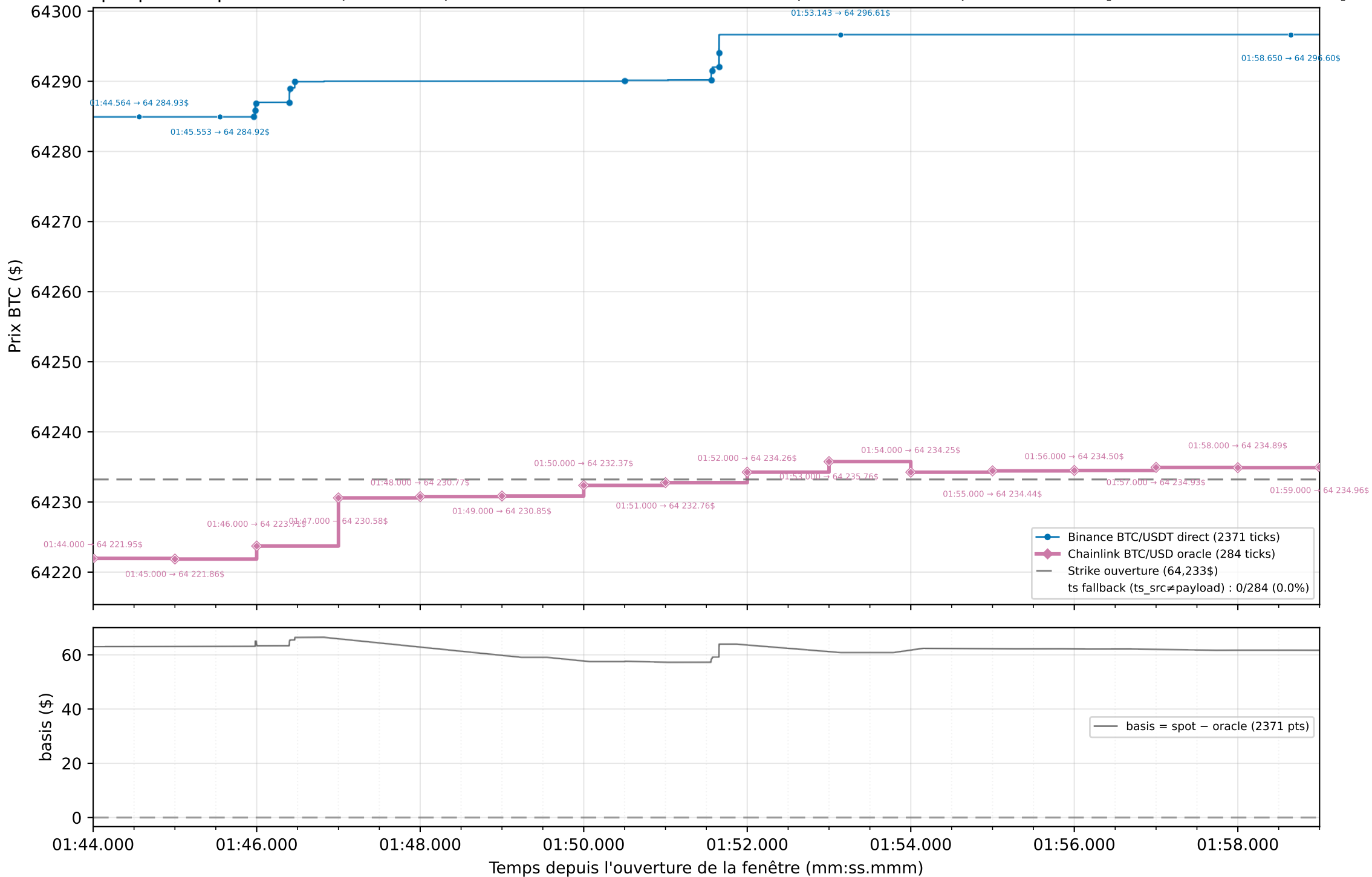
Graphique 2 : Spot Binance (flux direct) vs Oracle Chainlink — strike exact (dernier tick ≤ t0) — zoom 15 s [01:44.000 → 01:59.000]
