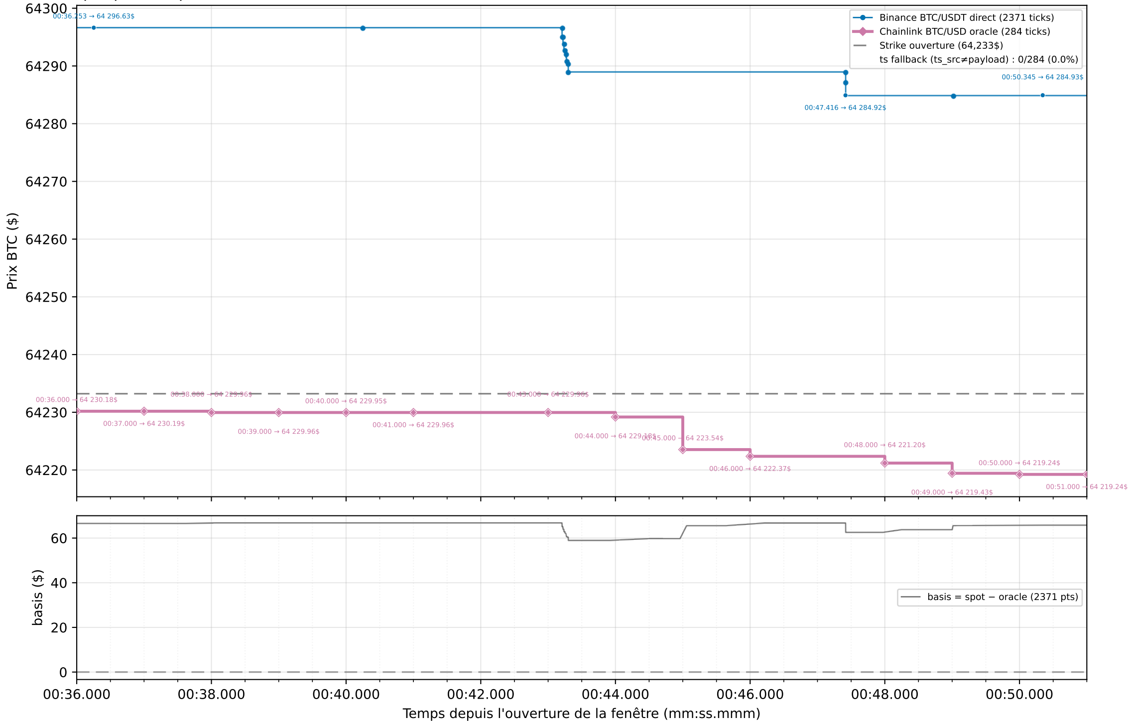
Graphique 2 : Spot Binance (flux direct) vs Oracle Chainlink — strike exact (dernier tick ≤ t0) — zoom 15 s [00:36.000 → 00:51.000]
