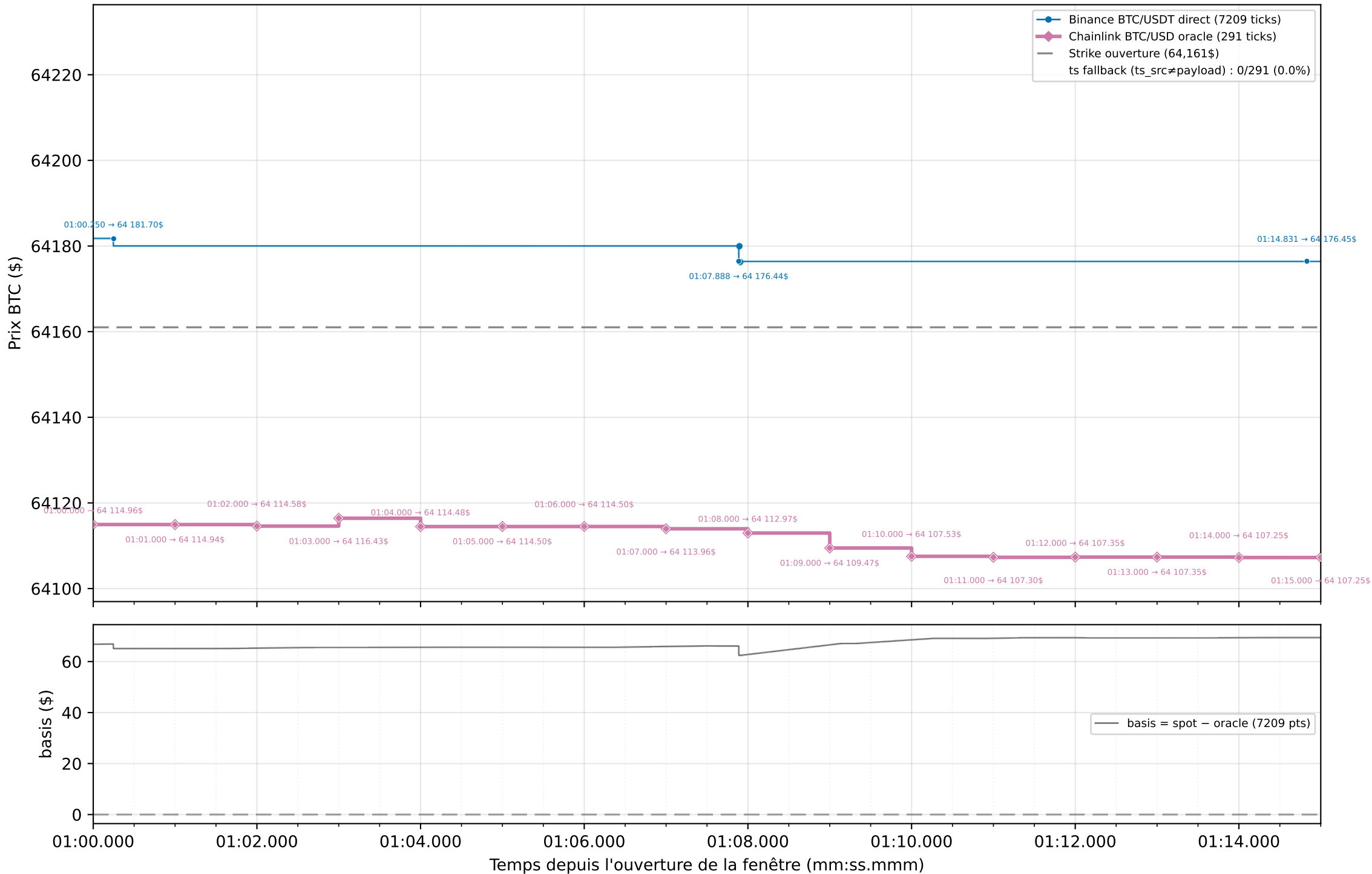
Graphique 2 : Spot Binance (flux direct) vs Oracle Chainlink — strike exact (dernier tick \leq t_0 ) — zoom 15 s [01:00.000 → 01:15.000]
