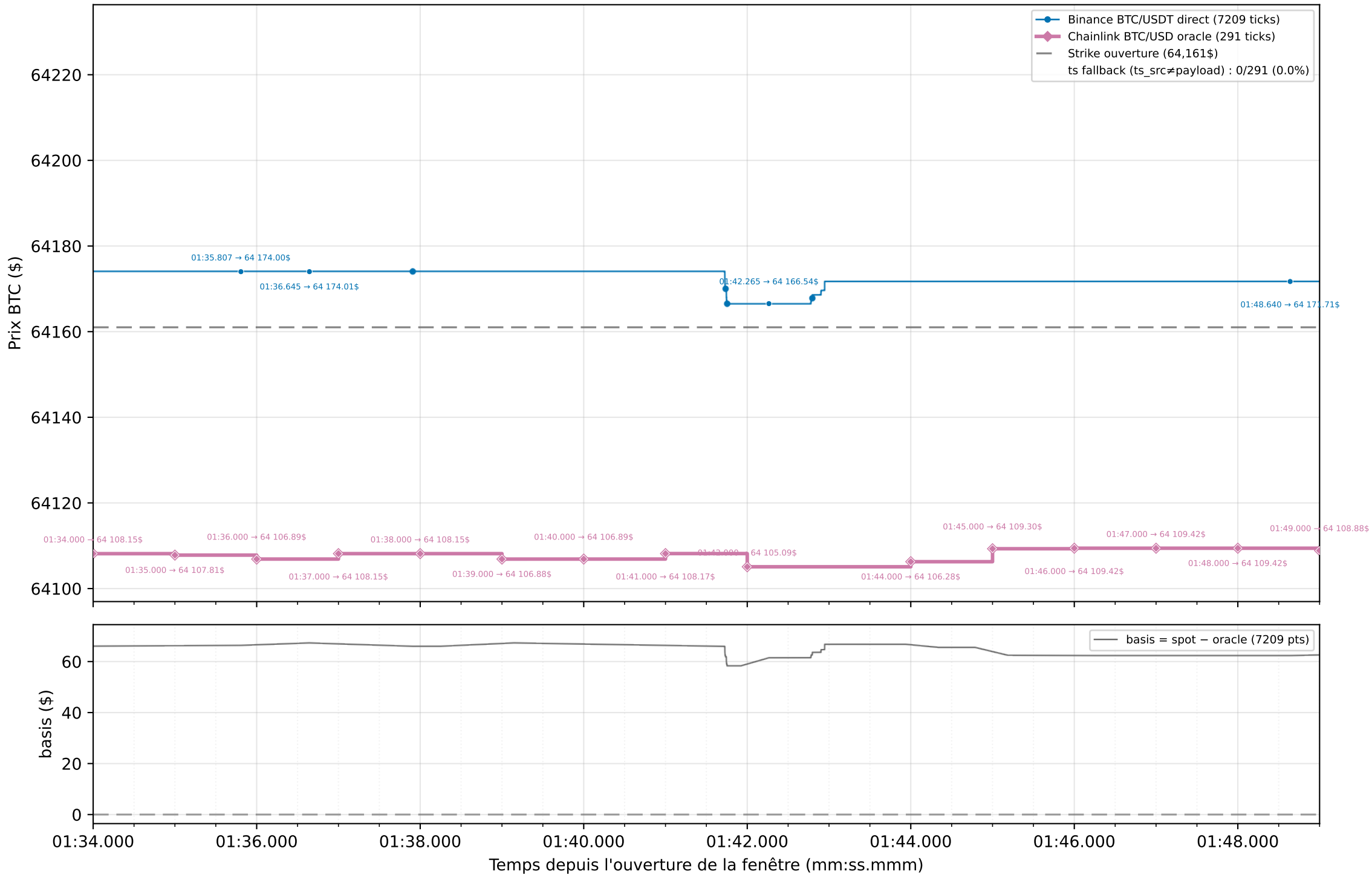
Graphique 2 : Spot Binance (flux direct) vs Oracle Chainlink — strike exact (dernier tick \leq t_0 ) — zoom 15 s [01:34.000 → 01:49.000]
