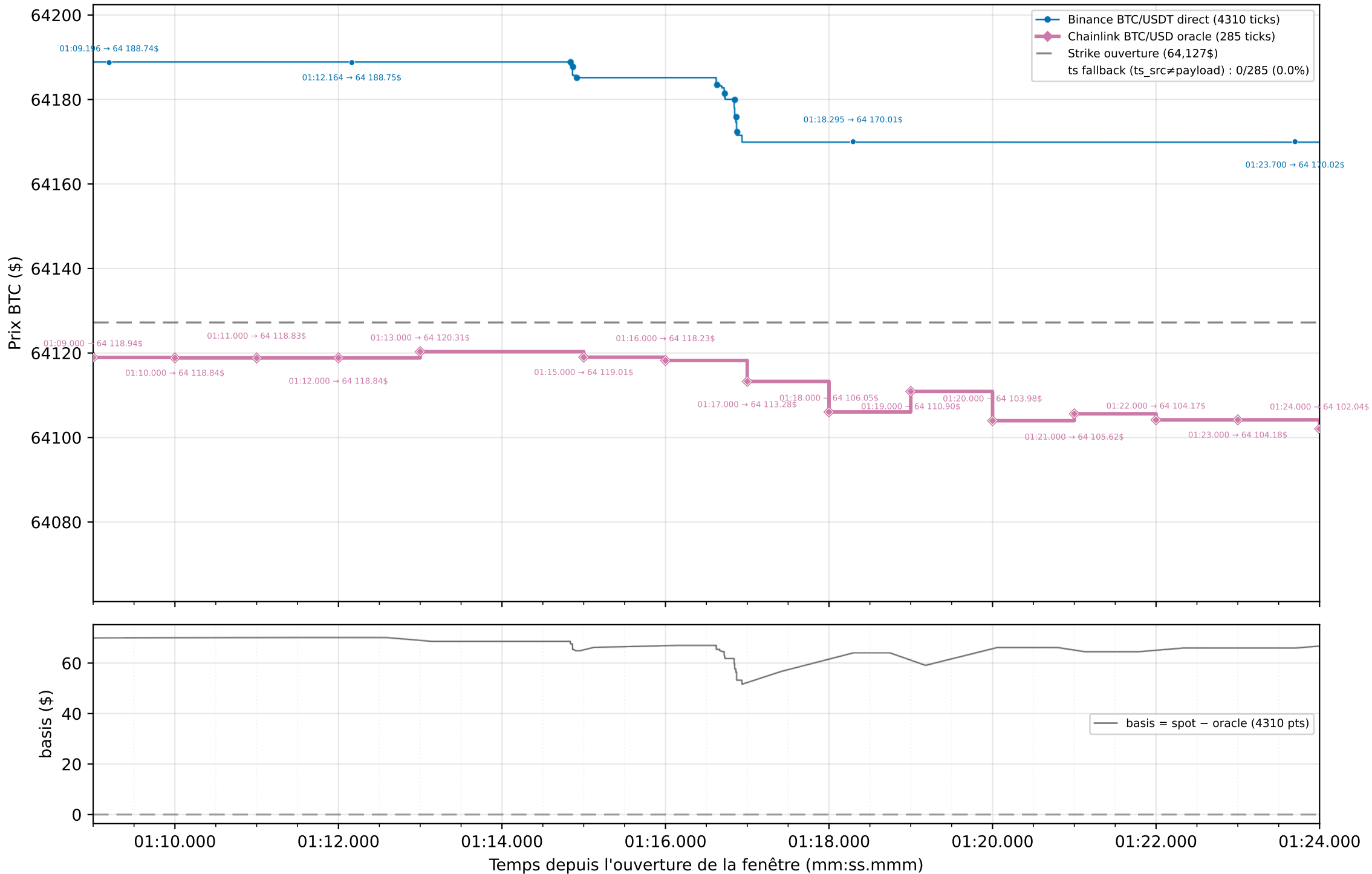
Graphique 2 : Spot Binance (flux direct) vs Oracle Chainlink — strike exact (dernier tick \leq t_0 ) — zoom 15 s [01:09.000 → 01:24.000]
